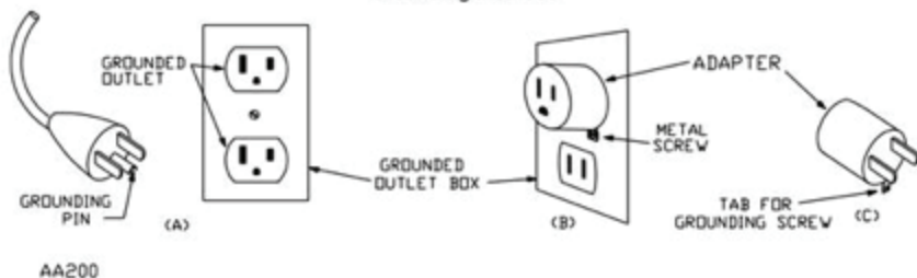
Figure 86.1 Grounding methods
